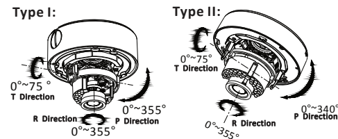
Figure 2-4 3-axis Adjustment
