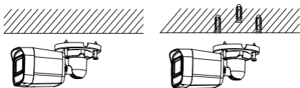
Figure 2-2 Attach the Camera to the Ceiling
