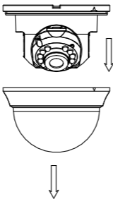
Figure 2-13 Remove the Bubble and the Black Liner
