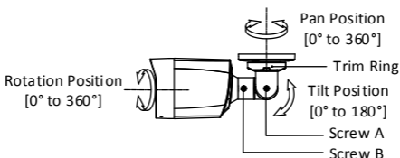
Figure 2-6 3-Axis Adjustment
