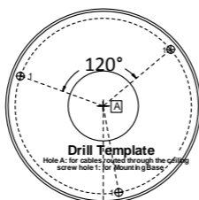
Figure 2-7 Drill Template
