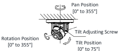
Figure 2-10 3-Axis Adjustment
