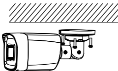
Figure 2-5 Attach the Camera to the Ceiling
