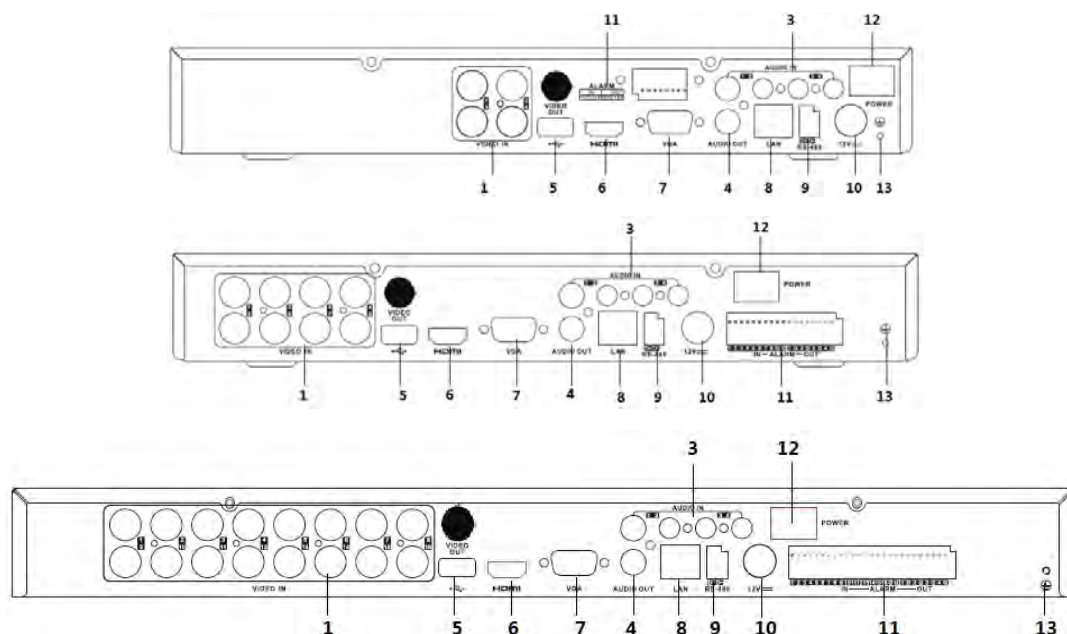
Figure 1. 7 4/8/16CH-FA Series
