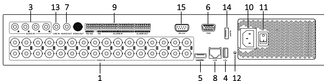
Figure 1. 10 24/32ch-FA Series
