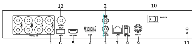
Figure 1. 4 Rear Panel
