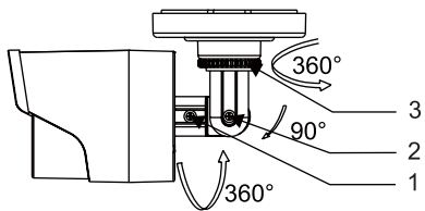
Figure 2-3 3-axis Adjustment
