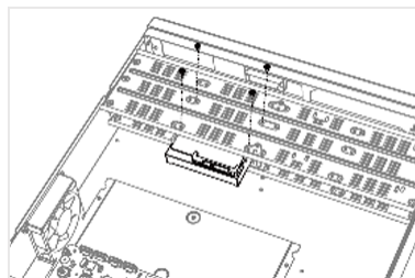
Figure 1-2 Fix HDD
