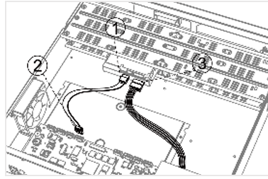
Figure 1-3 Connect Cable
