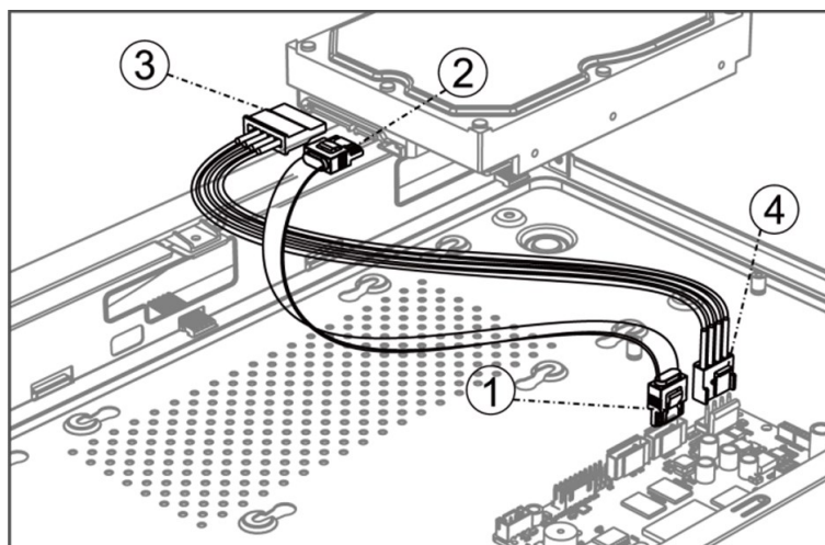
Figure 1-10 Connect Cables
