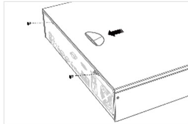
Figure 1-1 Remove Cover
