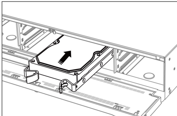
Figure 1-6 Insert HDD
