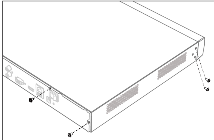
Figure 1-9 Remove Cover
